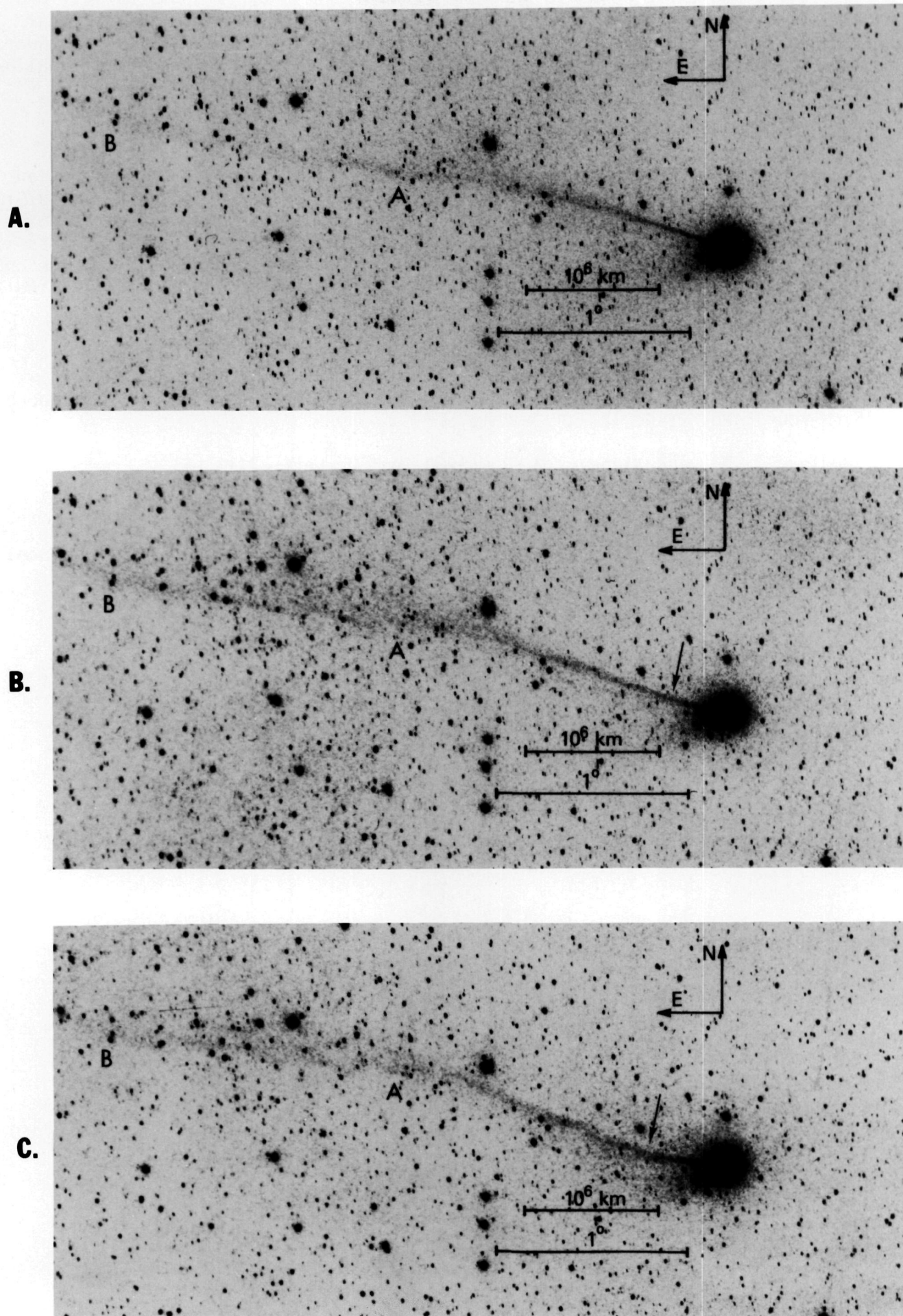
Figure 12. JOCR photographs of comet Bradfield on February 6, 1980. Midpoints of the exposures are: (a) 2^{\text{h}}32^{\text{m}}30^{\text{s}} UT; (b) 2^{\text{h}}48^{\text{m}}00^{\text{s}} UT; and (c) 3^{\text{h}}00^{\text{m}}00^{\text{s}} UT. See text for discussion.
